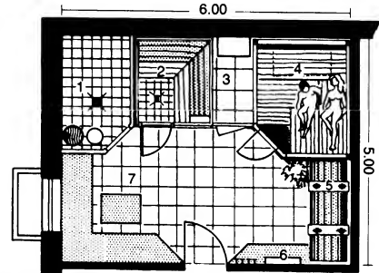
⑥ Sauna in the basement (35 m², 4–6 persons)
